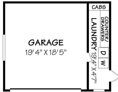
GARAGE / LAUNDRY
